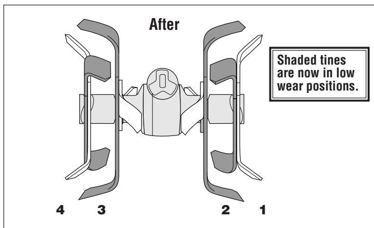
Figure 33: AFTER rotating gangs on cast iron holders.
