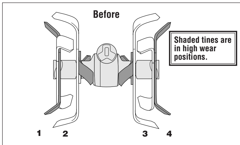
Figure 32: BEFORE rotating gangs on cast iron holders.
