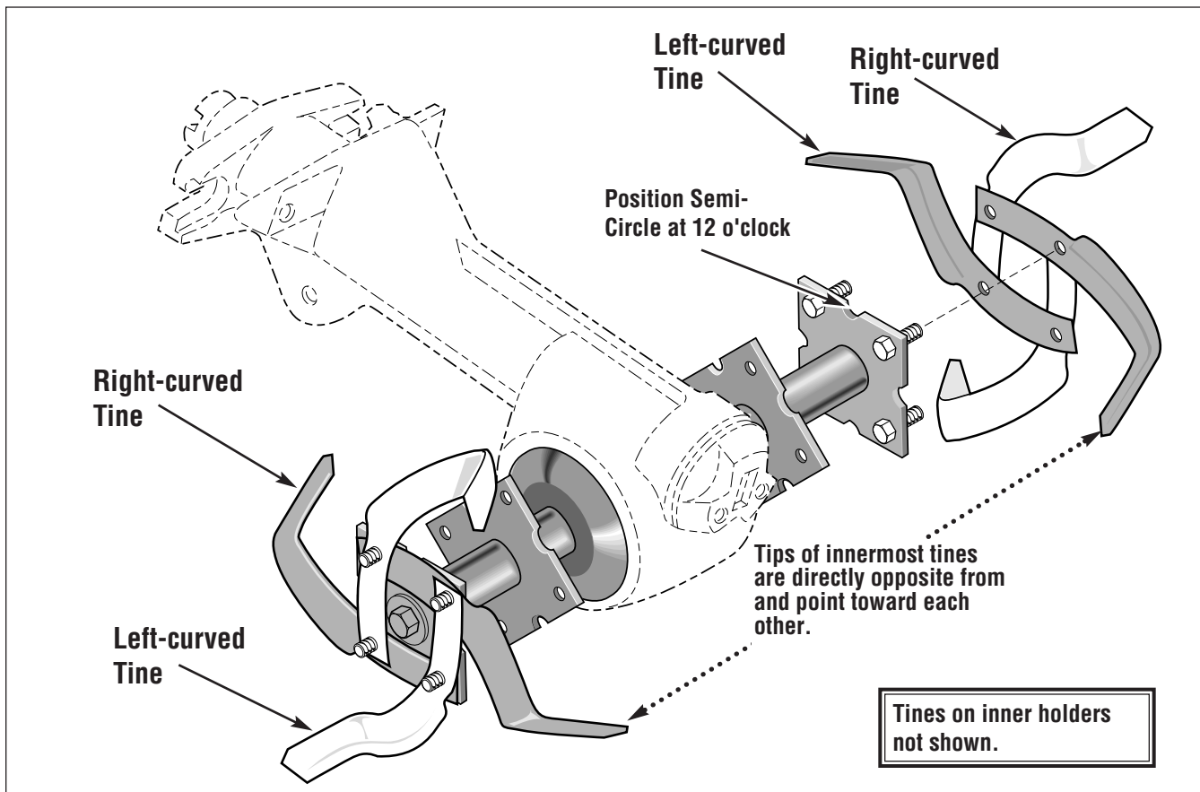
Figure 10: Installing tines on outer holders.
