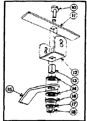
MAIN SUPPORT/YOKE ASSEMBLY PART # 1904522001
