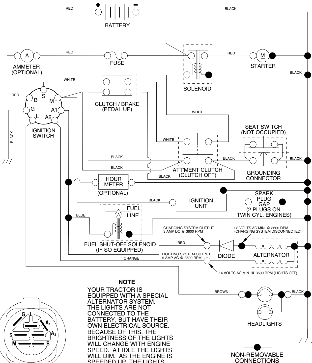
IGNITION SWITCH
