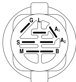
IGNITION SWITCH
