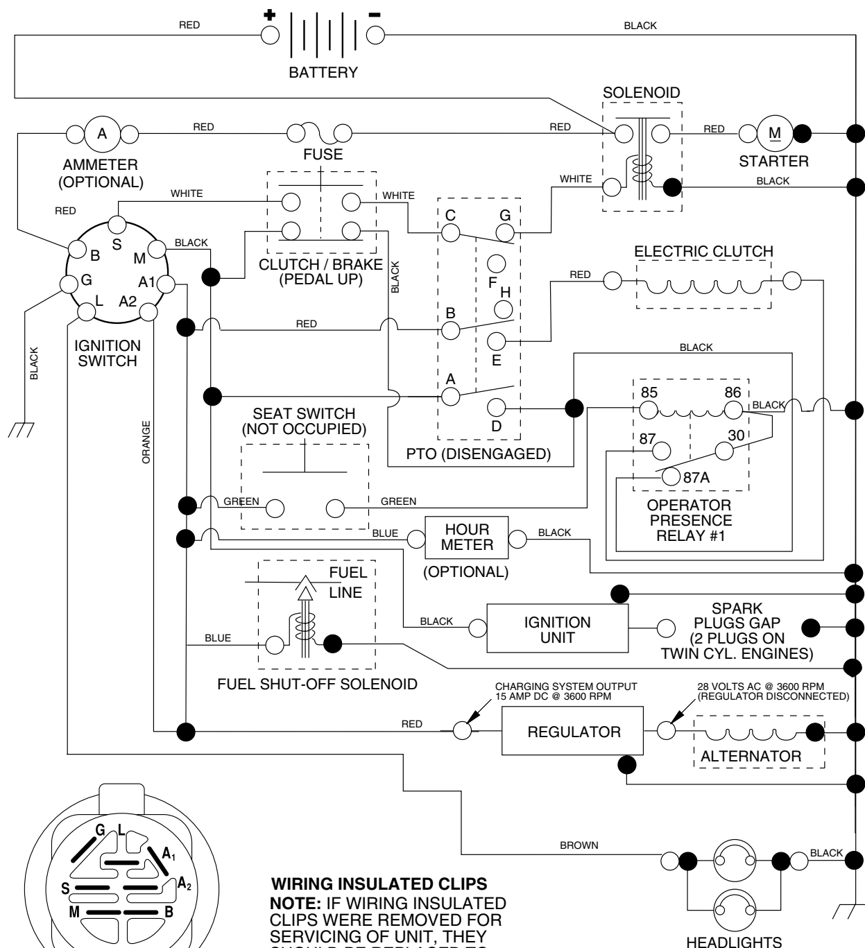
IGNITION SWITCH
