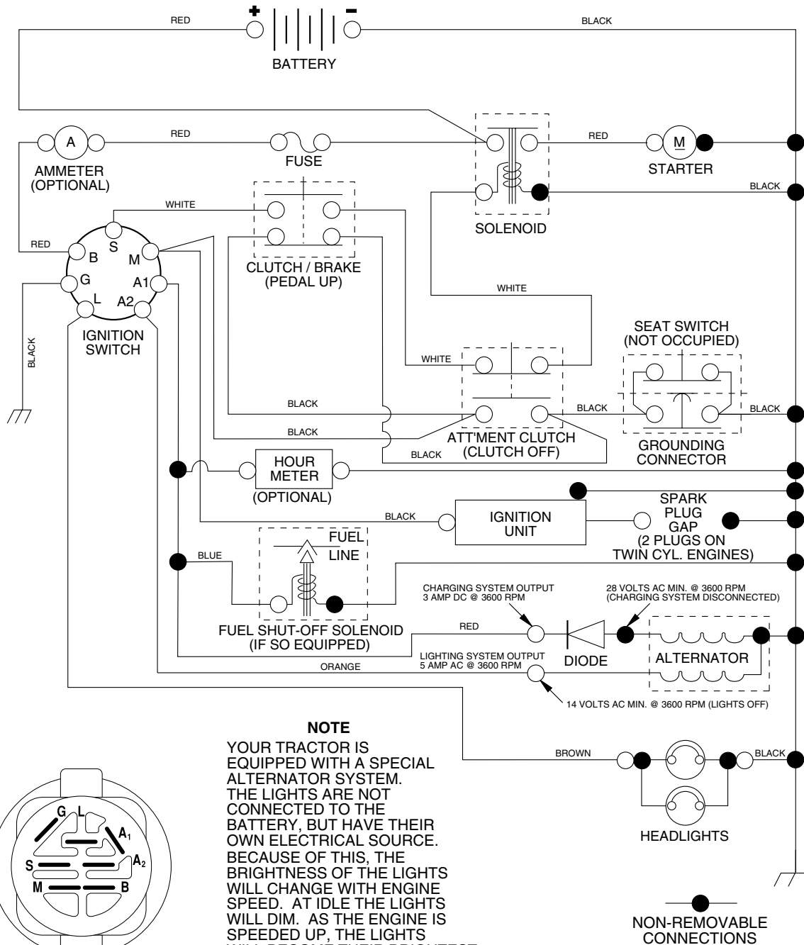
IGNITION SWITCH
