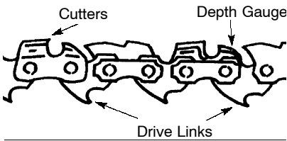
CUTTERS MUST FACE IN DIRECTION OF ROTATION
