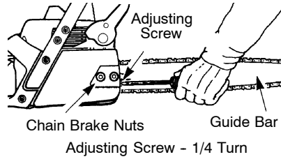
Adjusting Screw - 1/4 Turn
