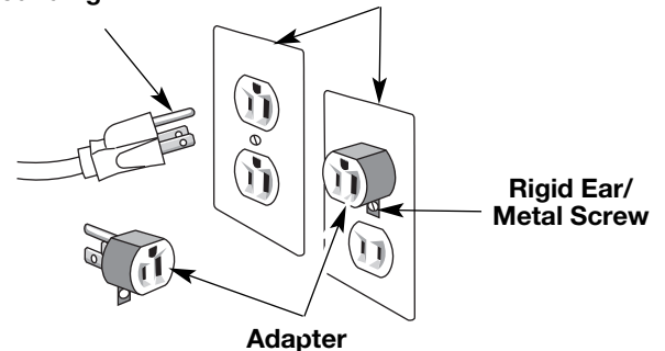
Grounding Pin
