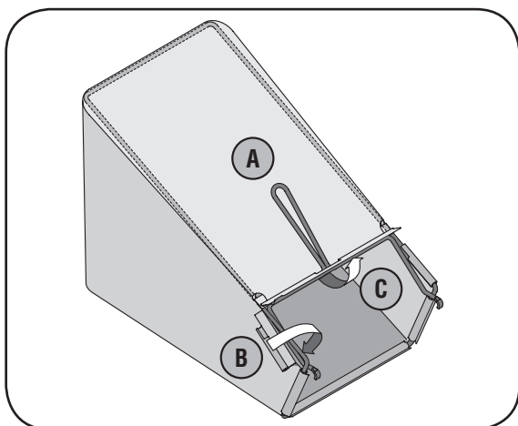
Figure 3-5: Assemble the grass catcher.
