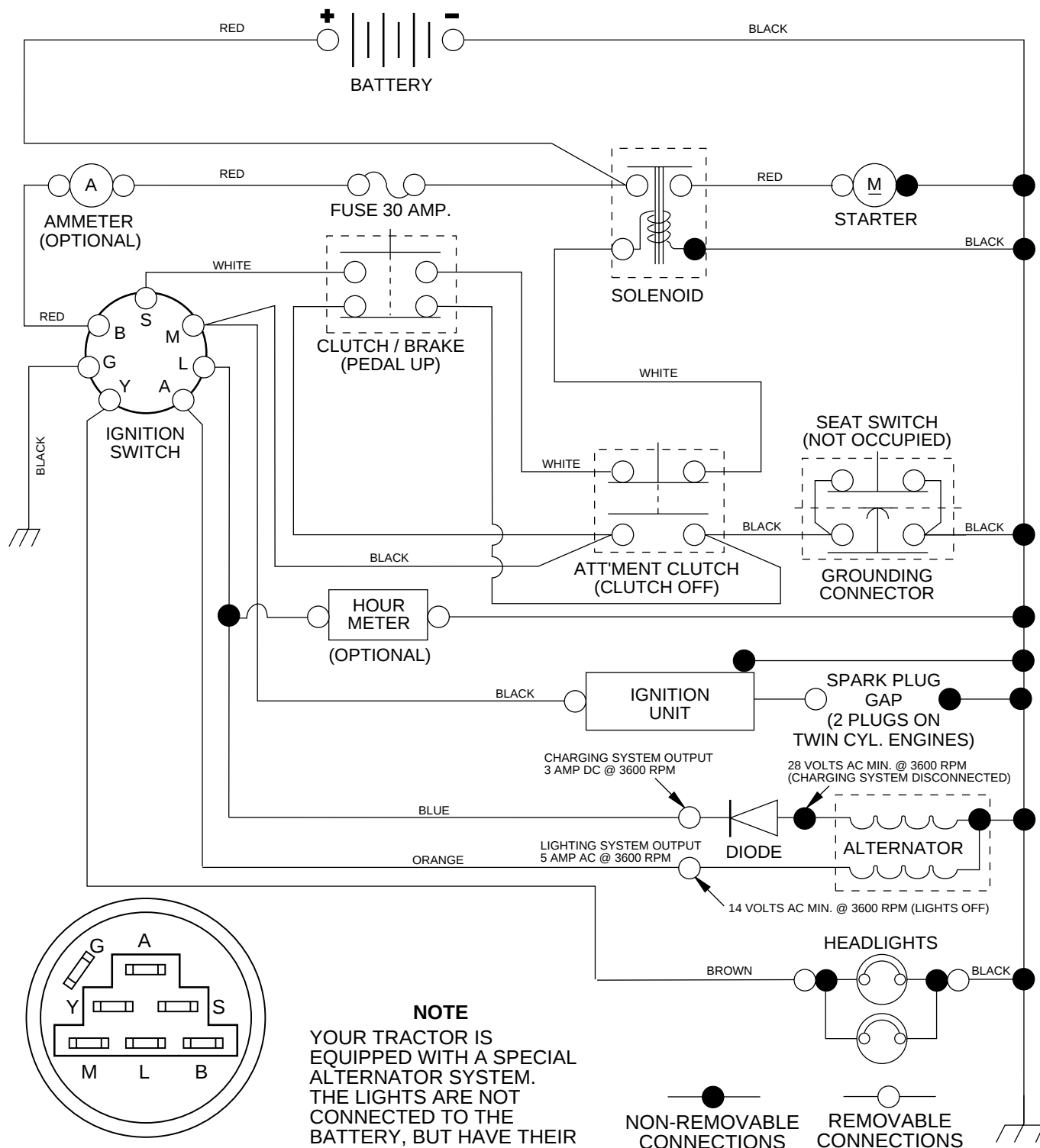
IGNITION SWITCH
