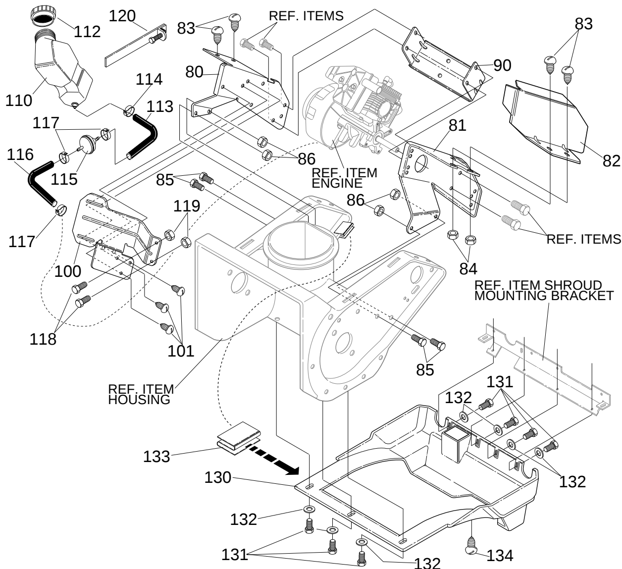
FRAME COMPONENTS REPAIR PARTS
