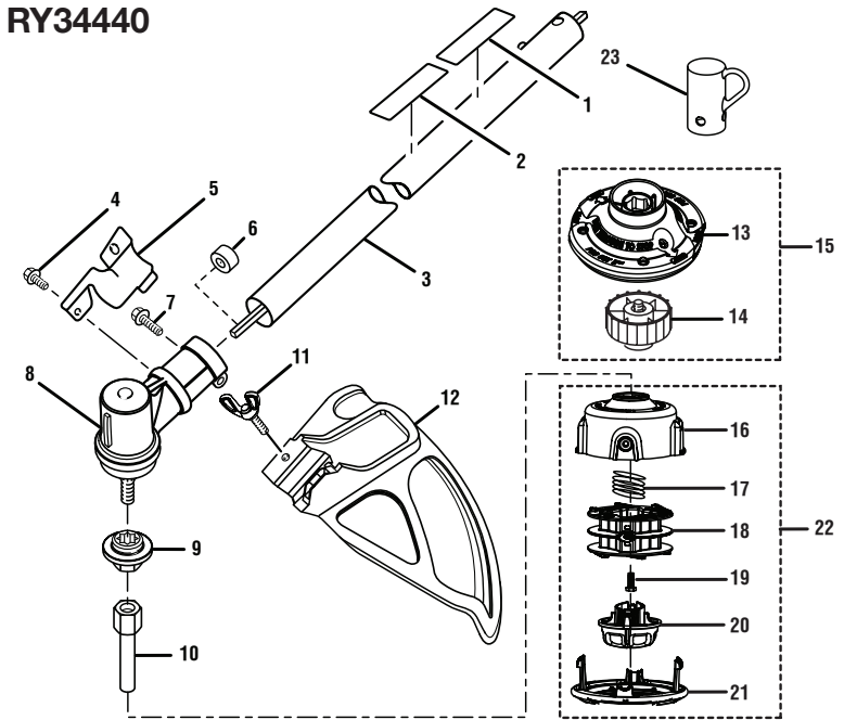
FIGURE C MODEL RY34440
