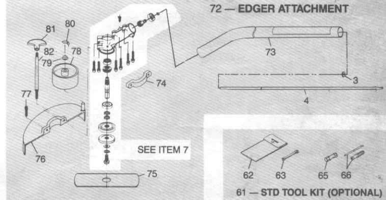
72 — EDGER ATTACHMENT
