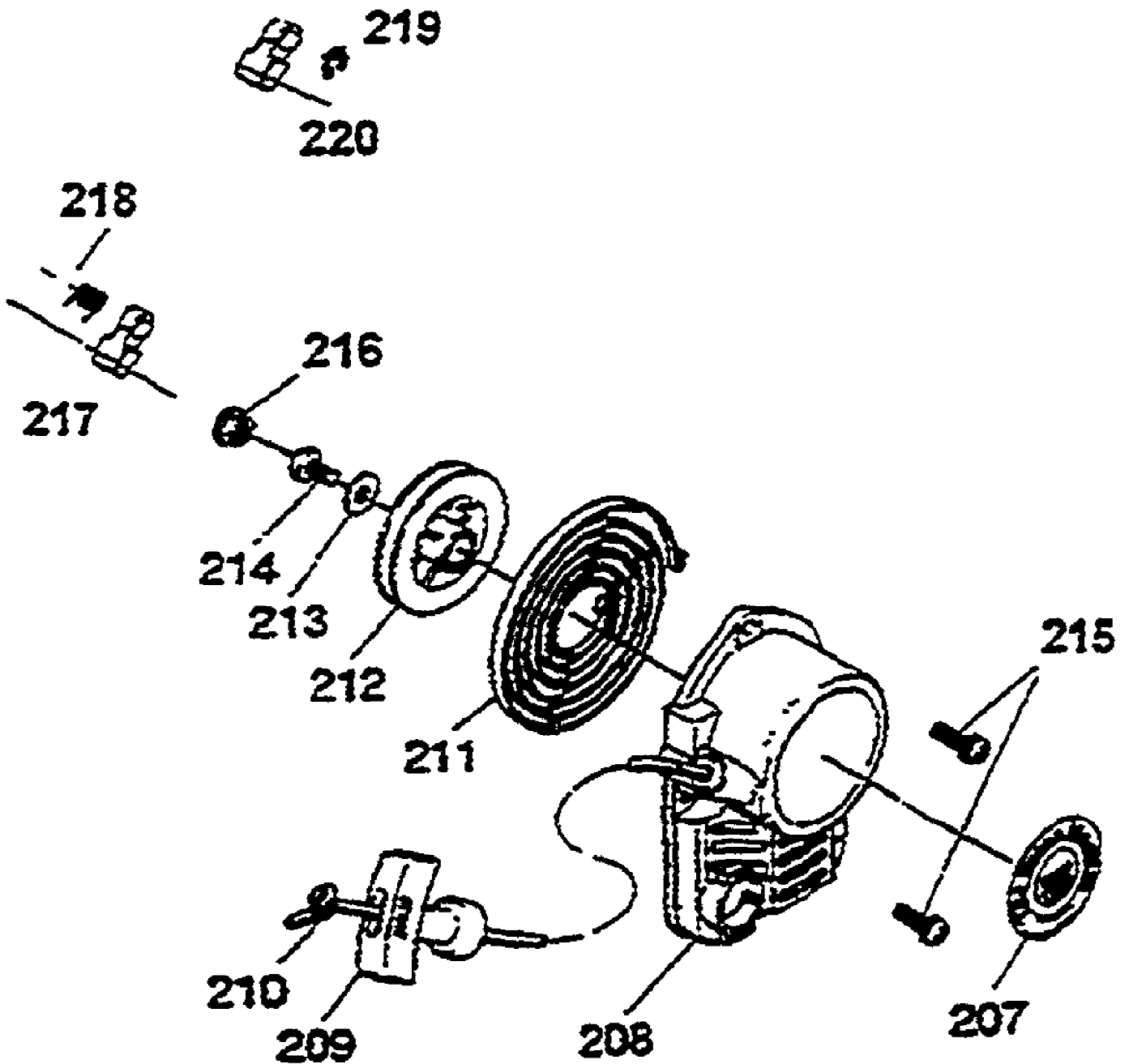
206 — STARTER ASSY
