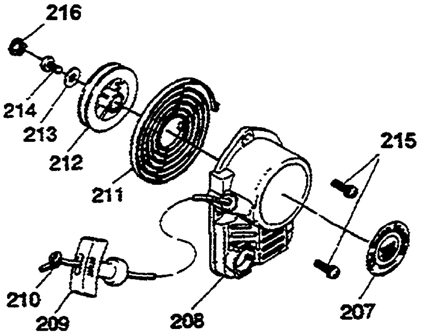
206 — STARTER ASSY
