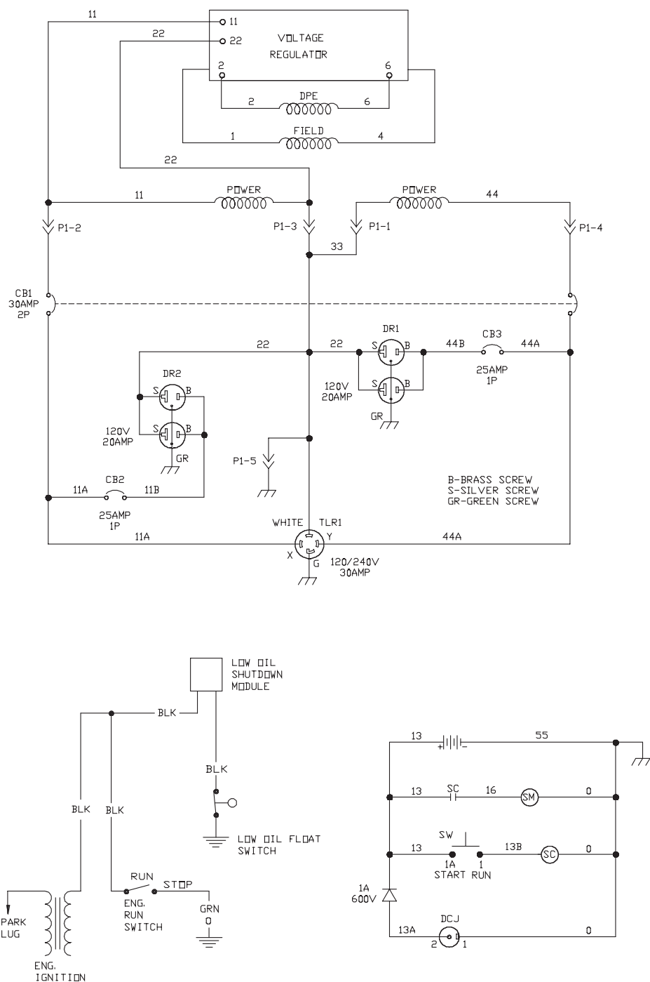
SCHEMATIC
