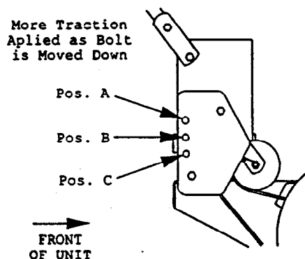
FIG. 16 DRIVE BELT TENSION ADJUSTMENT POSITIONS
