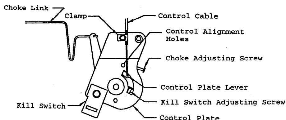
FIG 2 KOHLER SPEED CONTROL (THROTTLE CABLE HOOK-UP)
