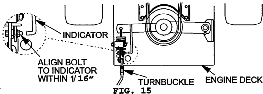
FIG. 15 BLADE ENGAGEMENT LINKAGE
