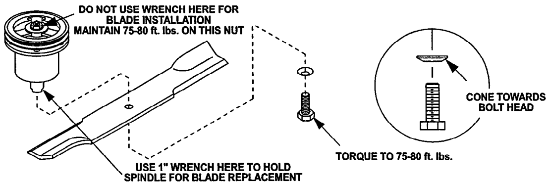
FIG. 13 BLADE BOLT INSTALLATION
