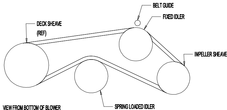
FIGURE 9 BELT ROUTING
