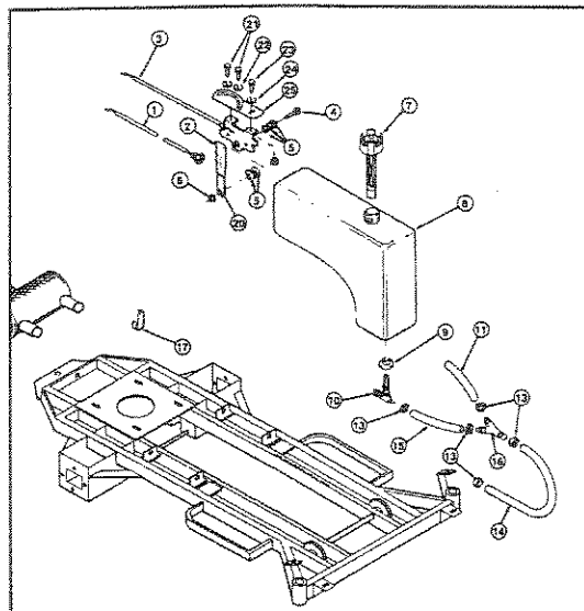
Fuel Strainer
