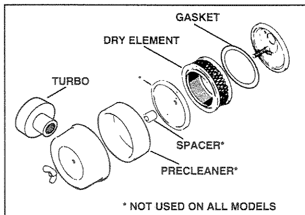
Air Cleaner
