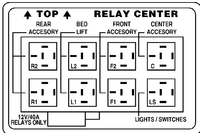
Relay Center
