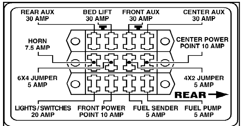
Fuse Box
