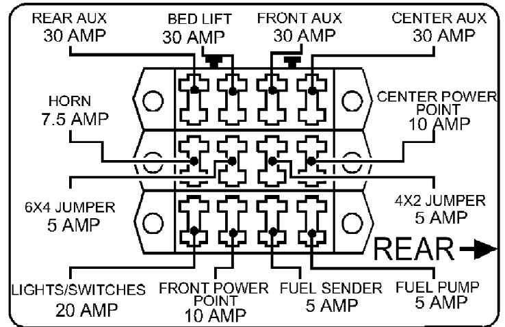
Fuse Box
