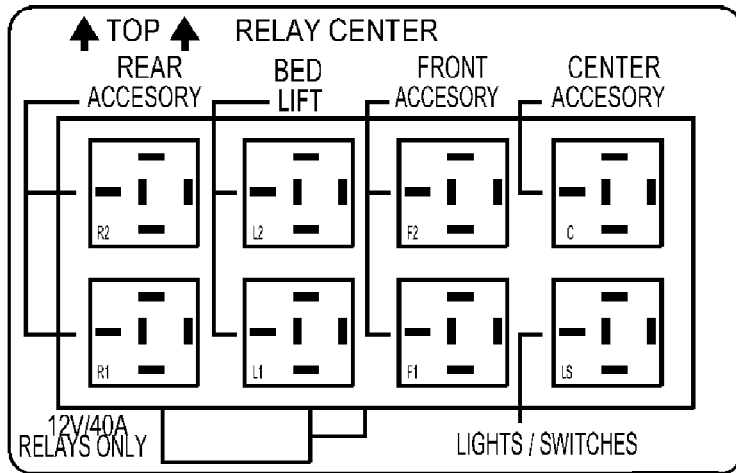
Relay Center
