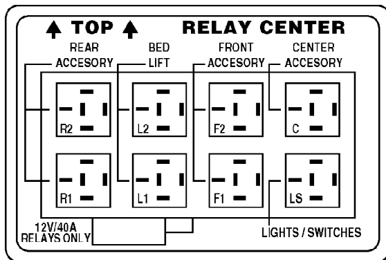
Relay Center
