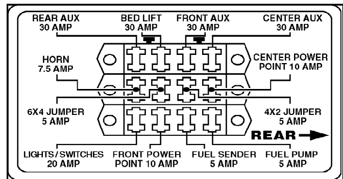
Fuse Box
