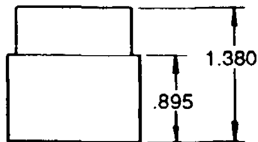
Bushing used in Clutch Assembly 717-3044
