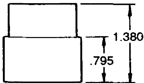
Bushing used in Clutch Assembly IH-144720-C91
