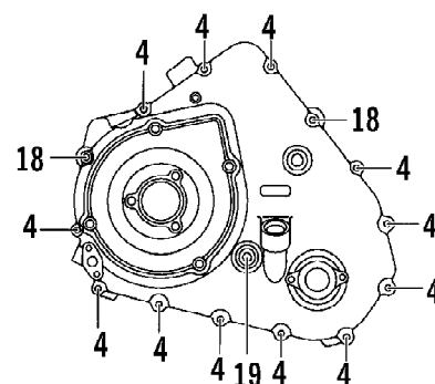
VIEW B
