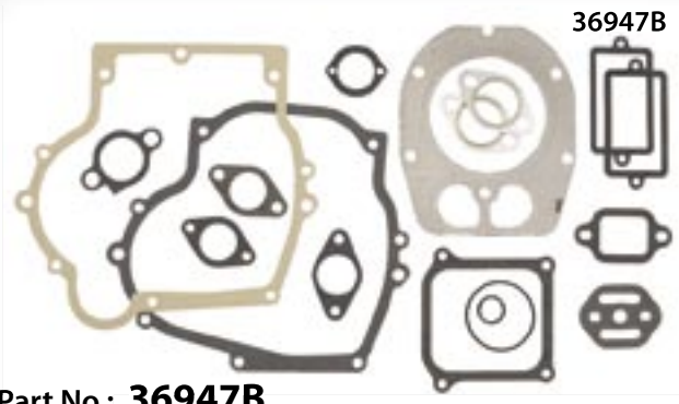
Part No.: 36947B Description: Gasket Set Models Used on: OH358, OHM120, OHSK, OHV, OV358
