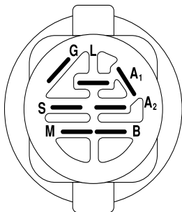
IGNITION SWITCH
