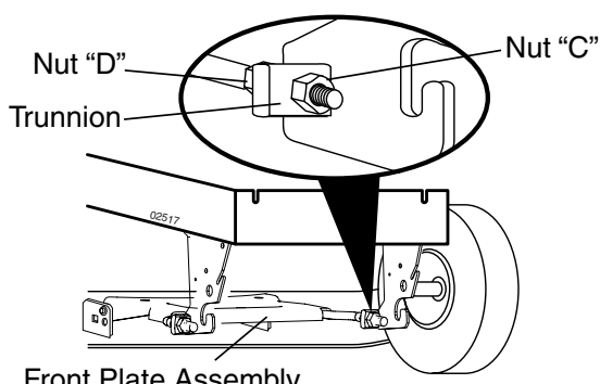
Front Plate Assembly
