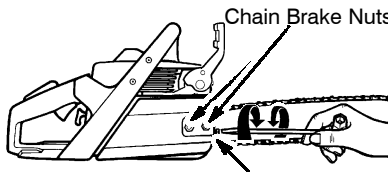
Adjusting screw
