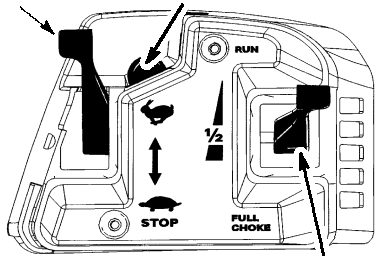
Choke Lever
