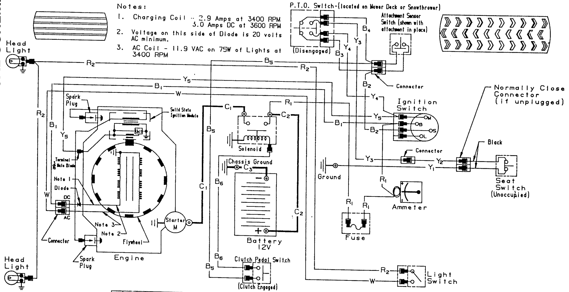
ELECTRICAL SCHEMATIC
