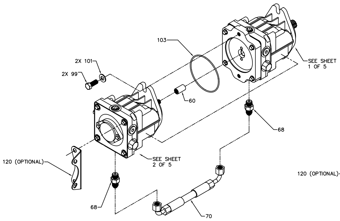
STD TANDEM W/ CHARGE PUMP
