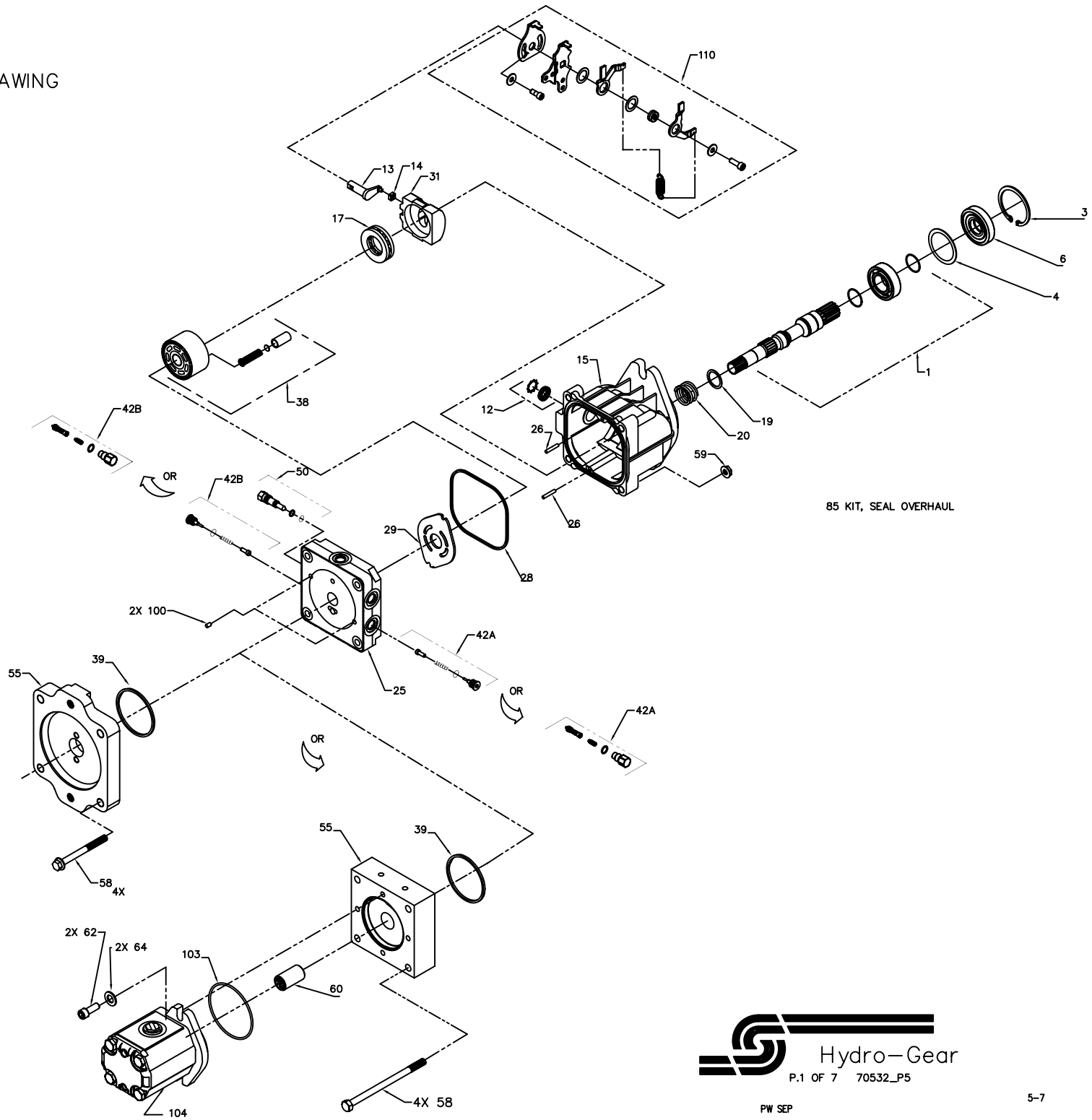
GEAR PUMP OPTION A
