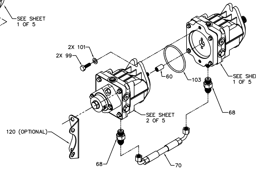
STD TANDEM W/ AUX PUMP
