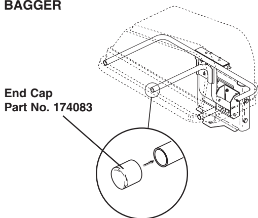
2-BIN BAGGER
