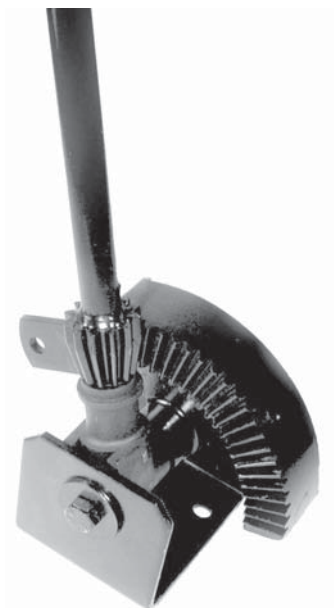
OLD STEERING ASSEMBLY
