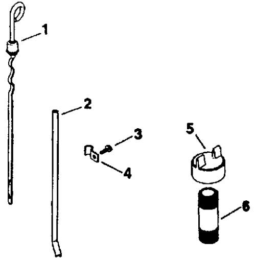
DIPSTICK
