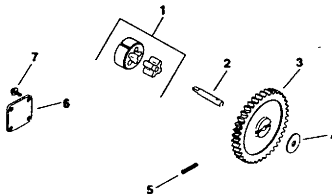
OIL PUMP
