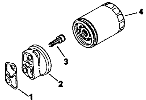
OIL FILTER
