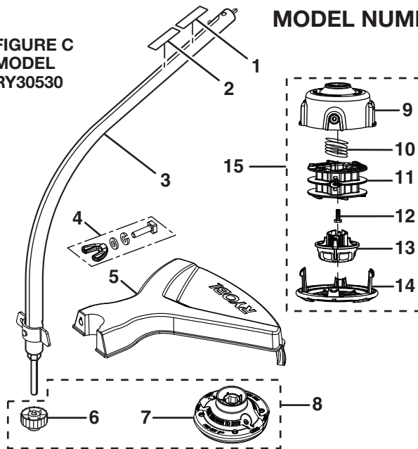
FIGURE C MODEL RY30550
