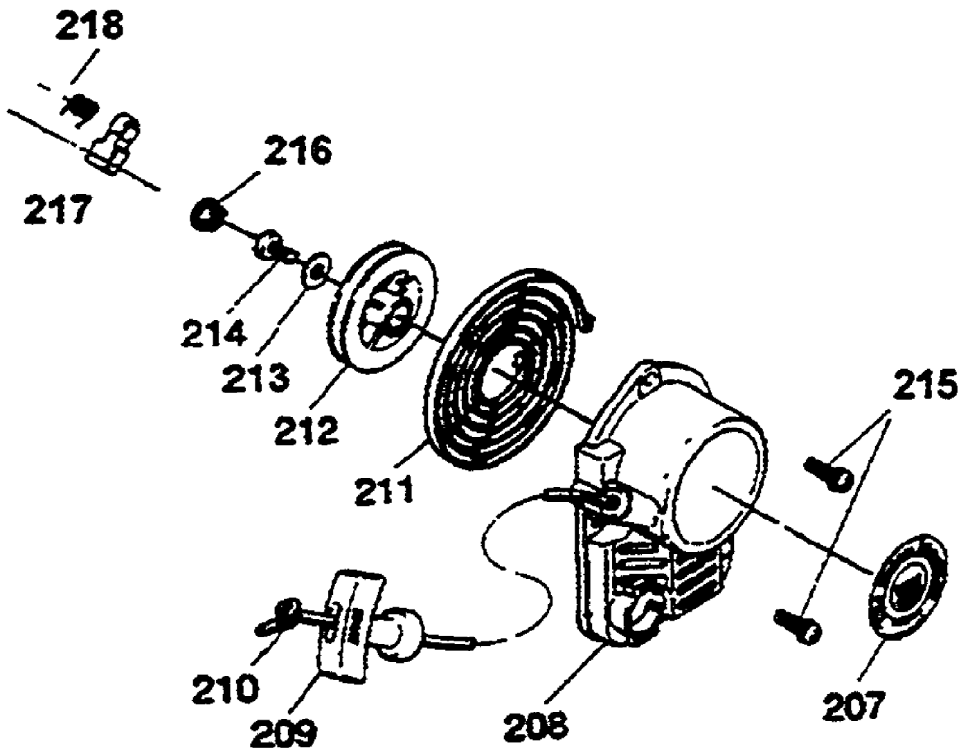
206 — STARTER ASSY
