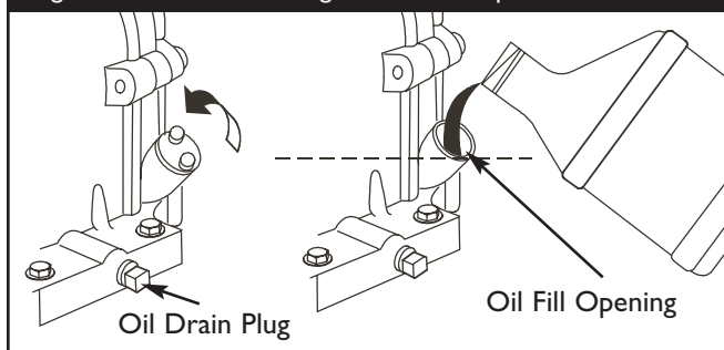
Figure 14 — Oil Drain Plug and Oil Fill Cap
