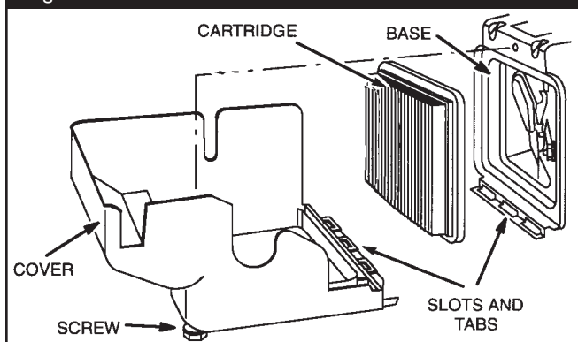
Figure 15 - Air Cleaner
