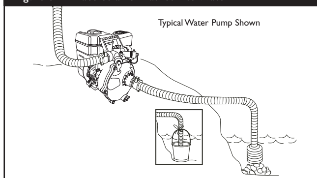
Figure 8 — Place Strainer Basket into Water
