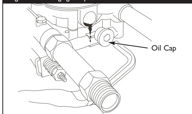
Figure 22 - Changing Pump Oil
