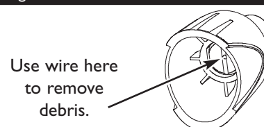
Figure 20 — Nozzle Maintenance
